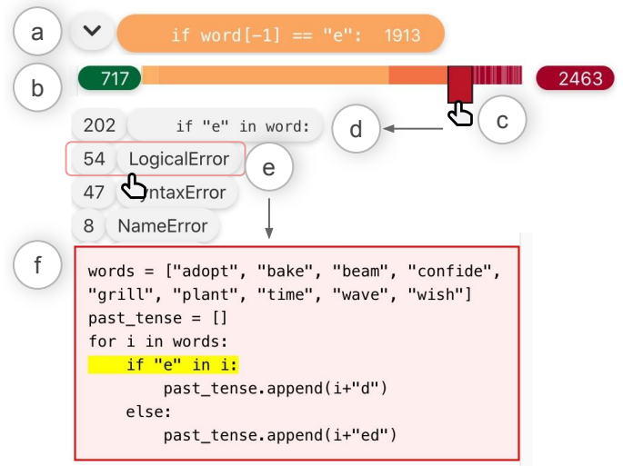
Figure 4: An example of how CFlow looks like without LLM determining line correctness. (a) is a collection of code lines that check the end of a word, and (b) is the correctness histogram. Upon selecting the prominent red block (c), users can view an example that incorrectly check the end of a word (d). By clicking on “LogicalError” (e), users are then able to explore detailed solutions (f).
